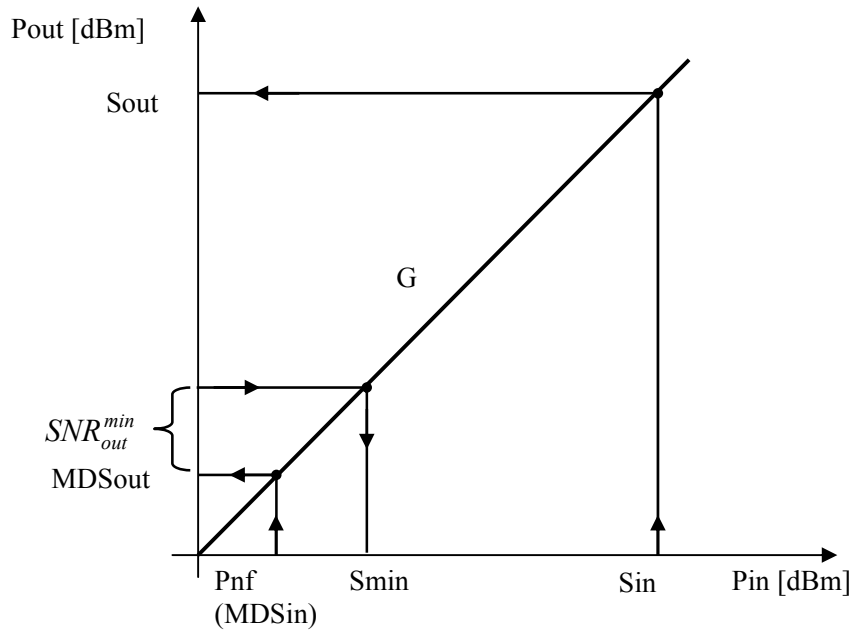
Fig.4.36. Definirea MDS_{out} .
